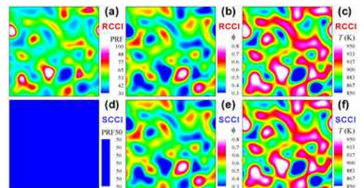
Fig. 2 Initial PRF, equivalence ratio, and temperature fields of (a–c) RCCI and (d–f) SCCI configuration for Case 5 and Case 8.
