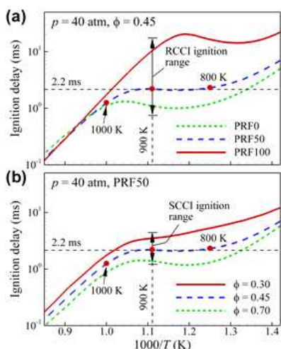
Fig. 3 0-D ignition delays of PRF/air mixtures as a function of initial temperature for (a) different PRFs and (b) different \phi at p_0 = 40\text{atm} .
