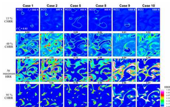
Fig. 5 Isocontours of normalized HRR for the cases with T_0 = 800 K (Case 1-2), T_0 = 900 K (Case 5 & 8), and T_0 = 1000 K (Case 9-10).
