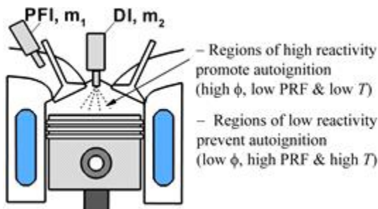
Fig. 1 RCCI operating concept. m_1 and m_2 are the mass fraction of low- and high-reactivity fuel.
