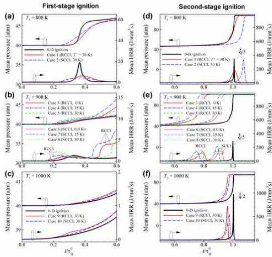
Fig. 4 Temporal evolutions of the mean pressure and mean HRR for the cases with T_0 = 800 K (a & d), T_0 = 900 K (b & e), and T_0 = 1000 K (c & f) during the first- (left) and second-stage (right) ignition.
